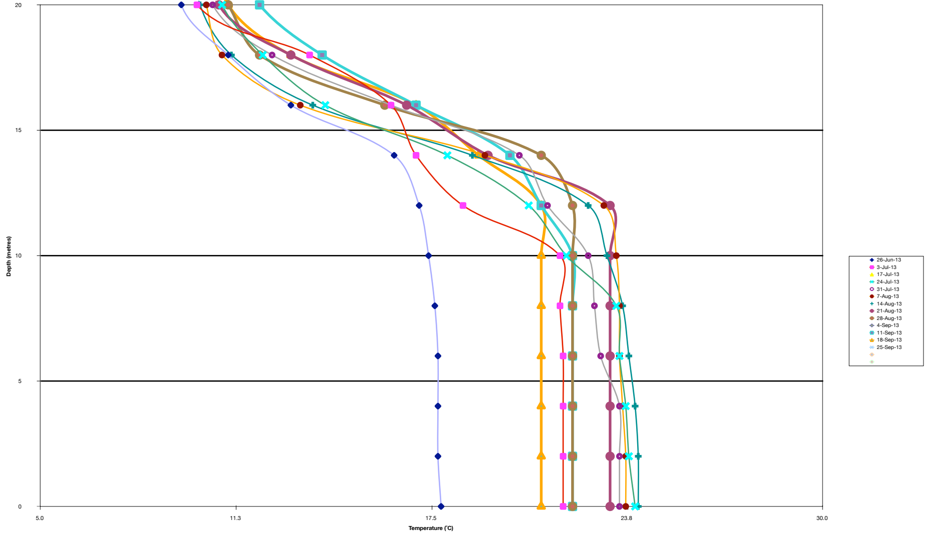
Osoyoos Lake (at White Sands) - Temperature Profiles 2013
