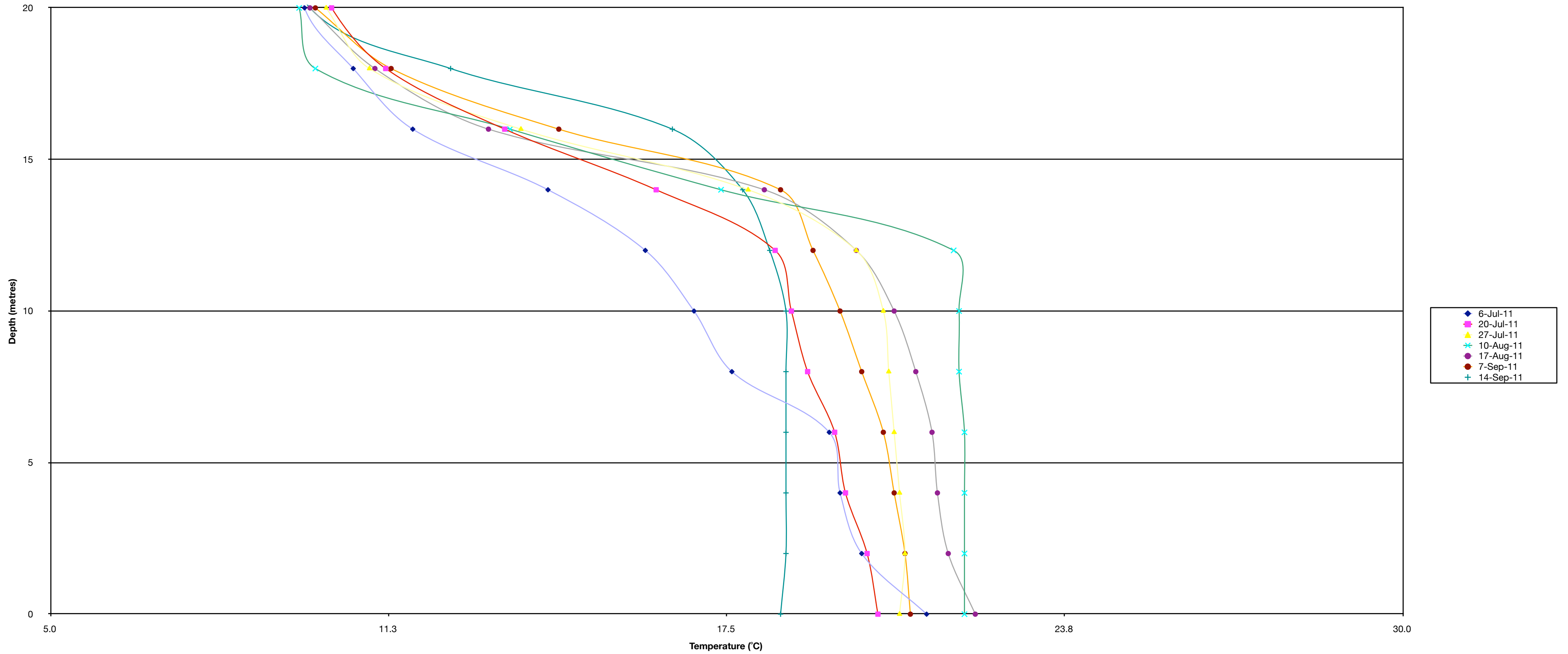
Osoyoos Lake (at White Sands) - Temperature Profiles 2011
