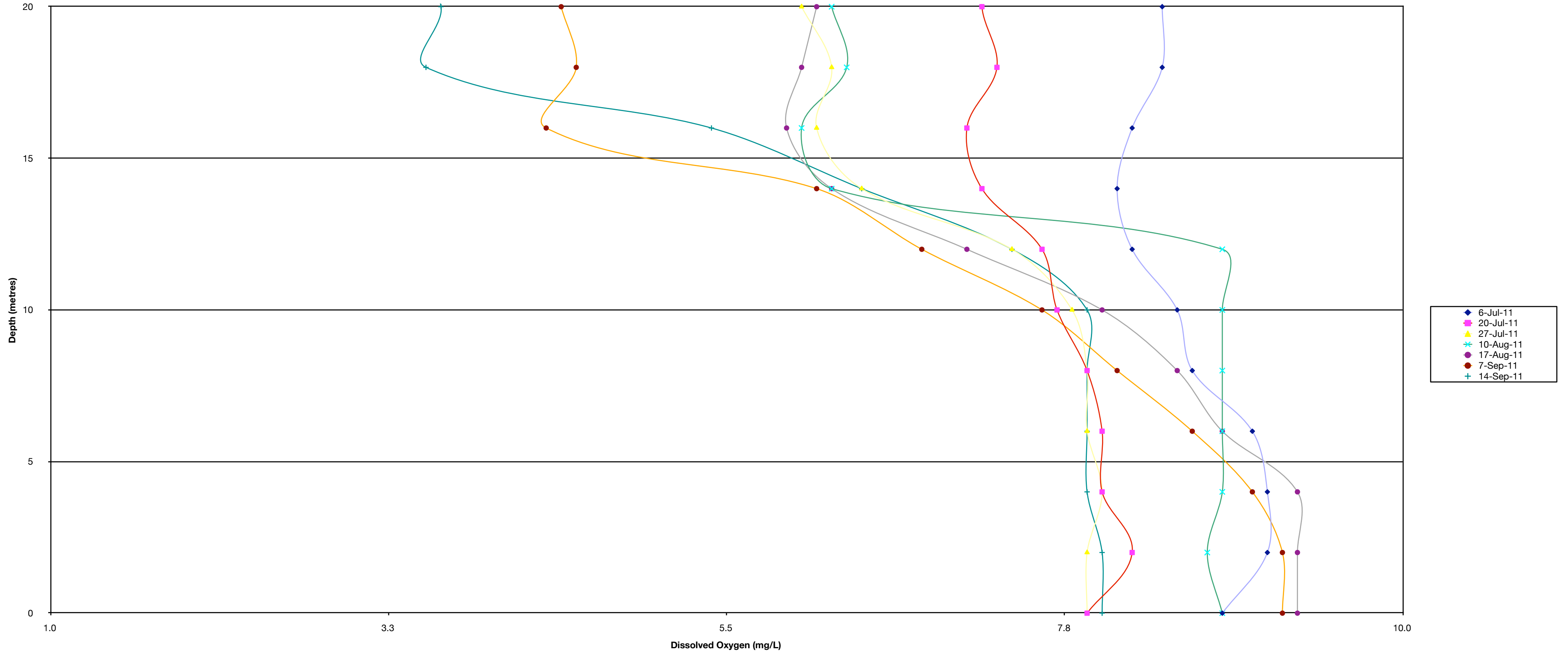
Osoyoos Lake (at White Sands) - Oxygen Profiles 2011
