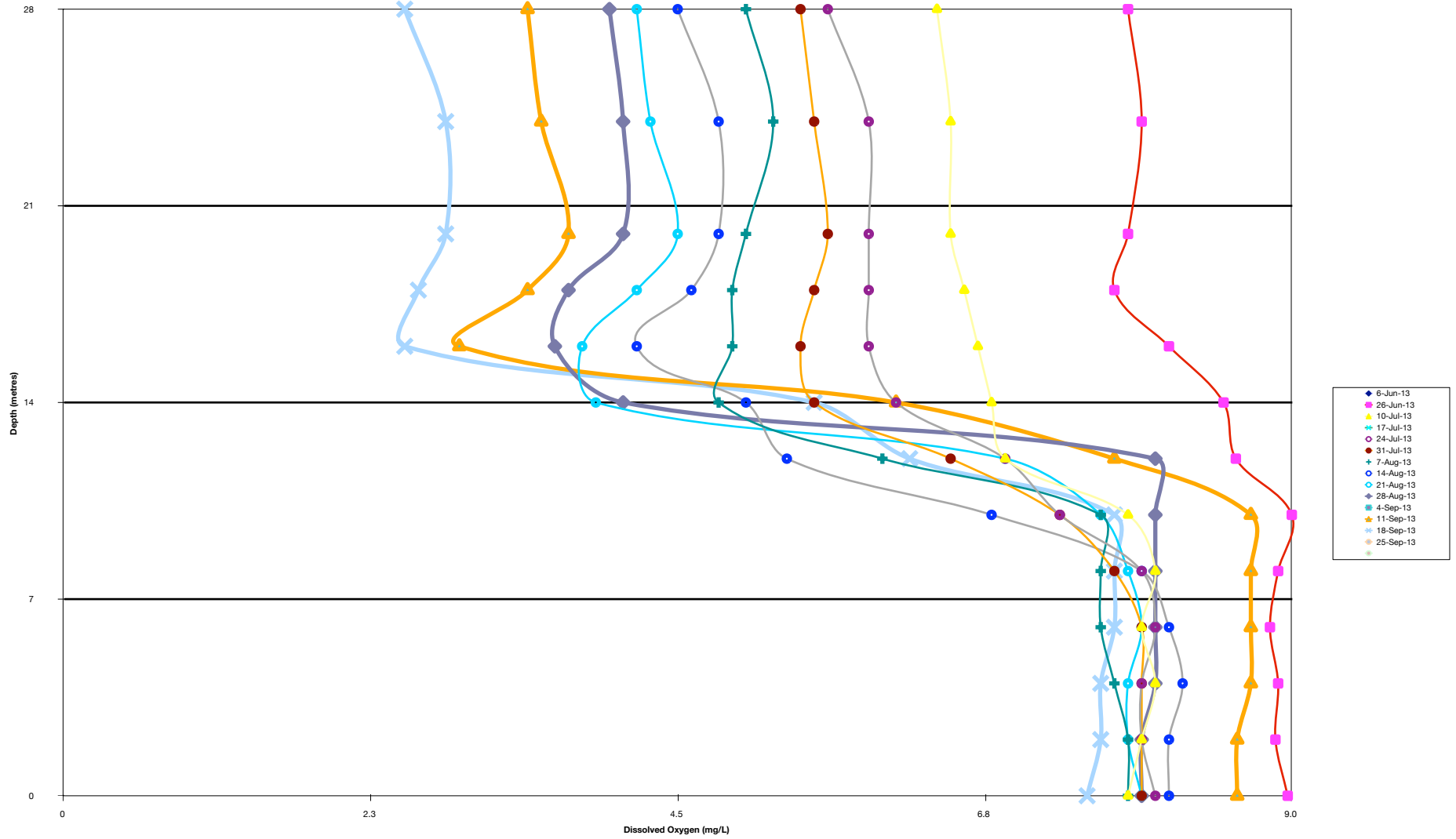
Osoyoos Lake (at Packinghouse) - Oxygen Profiles 2013
