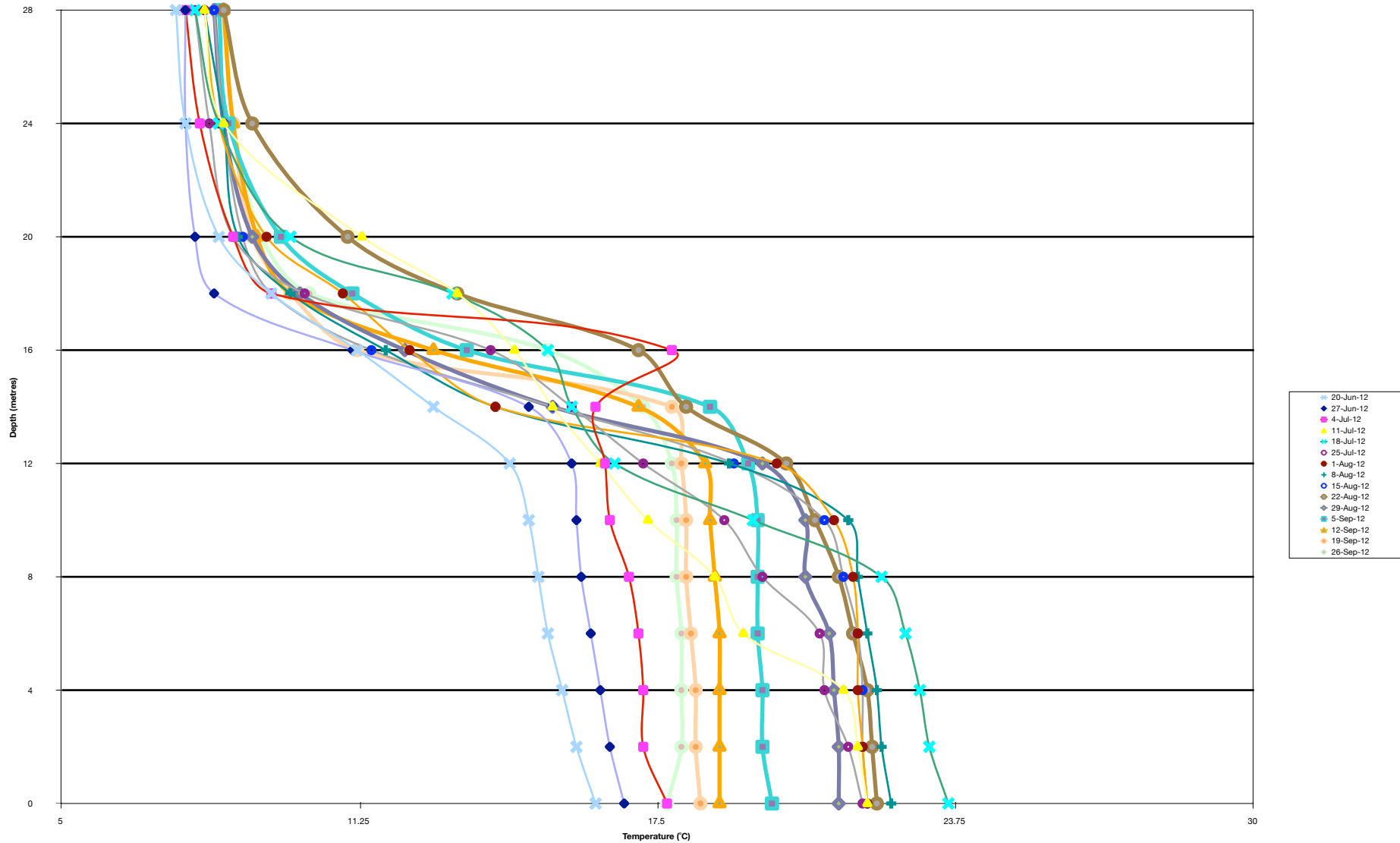
Osoyoos Lake (at North End) - Temperature Depth Profiles 2012
