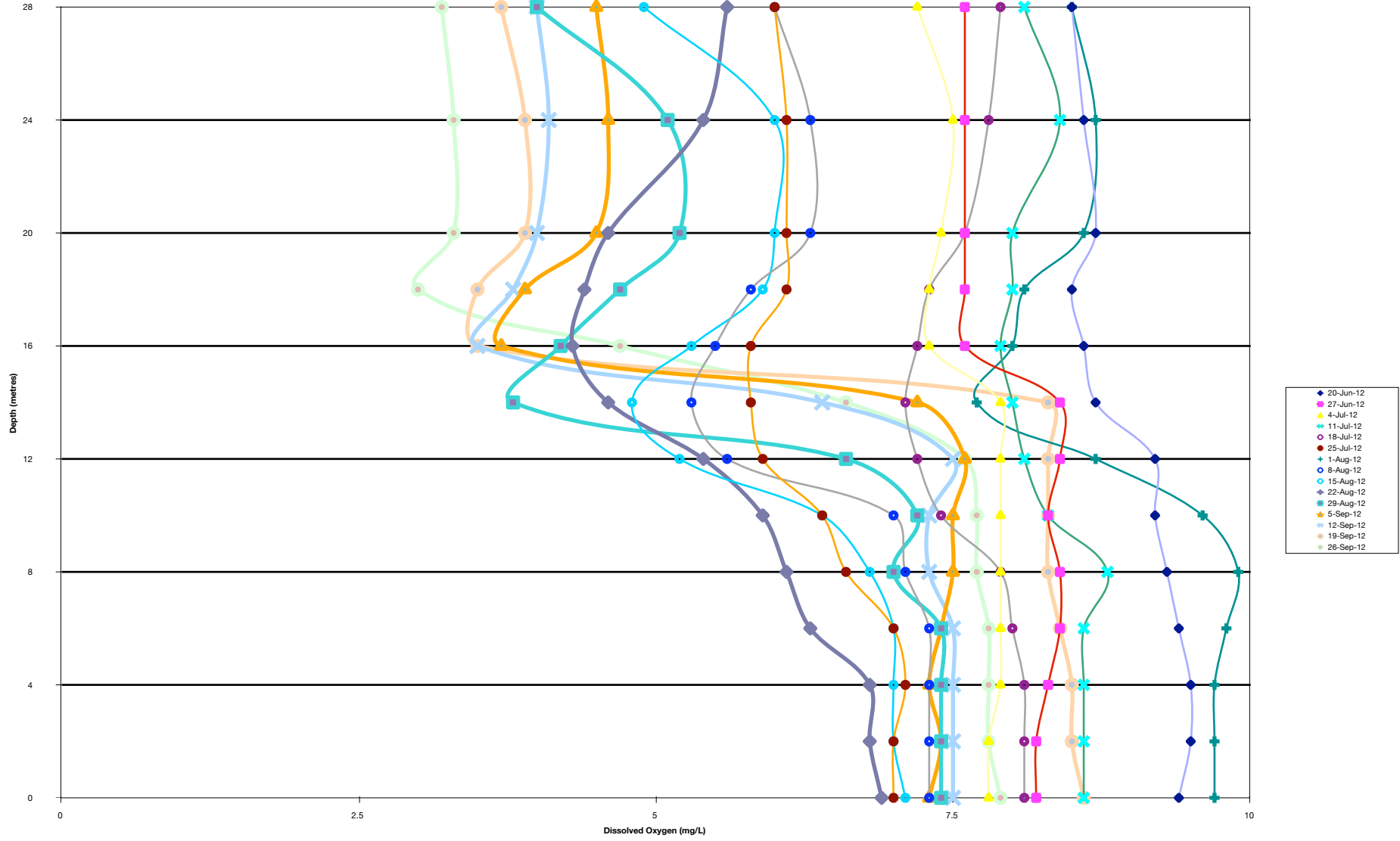
Osoyoos Lake (at North End) - Oxygen Profiles 2012
