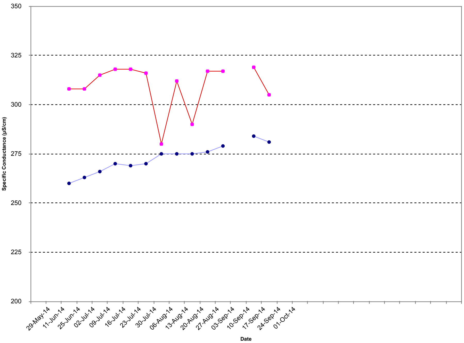
Osoyoos Lake (at Central Basin) - Specific Conductance
