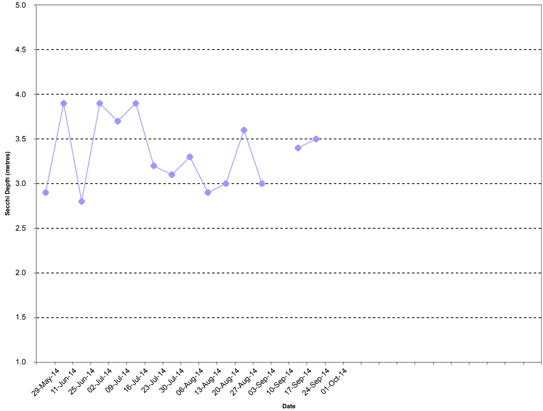
Osoyoos Lake (at Central Basin) - Secchi Depth 2014
