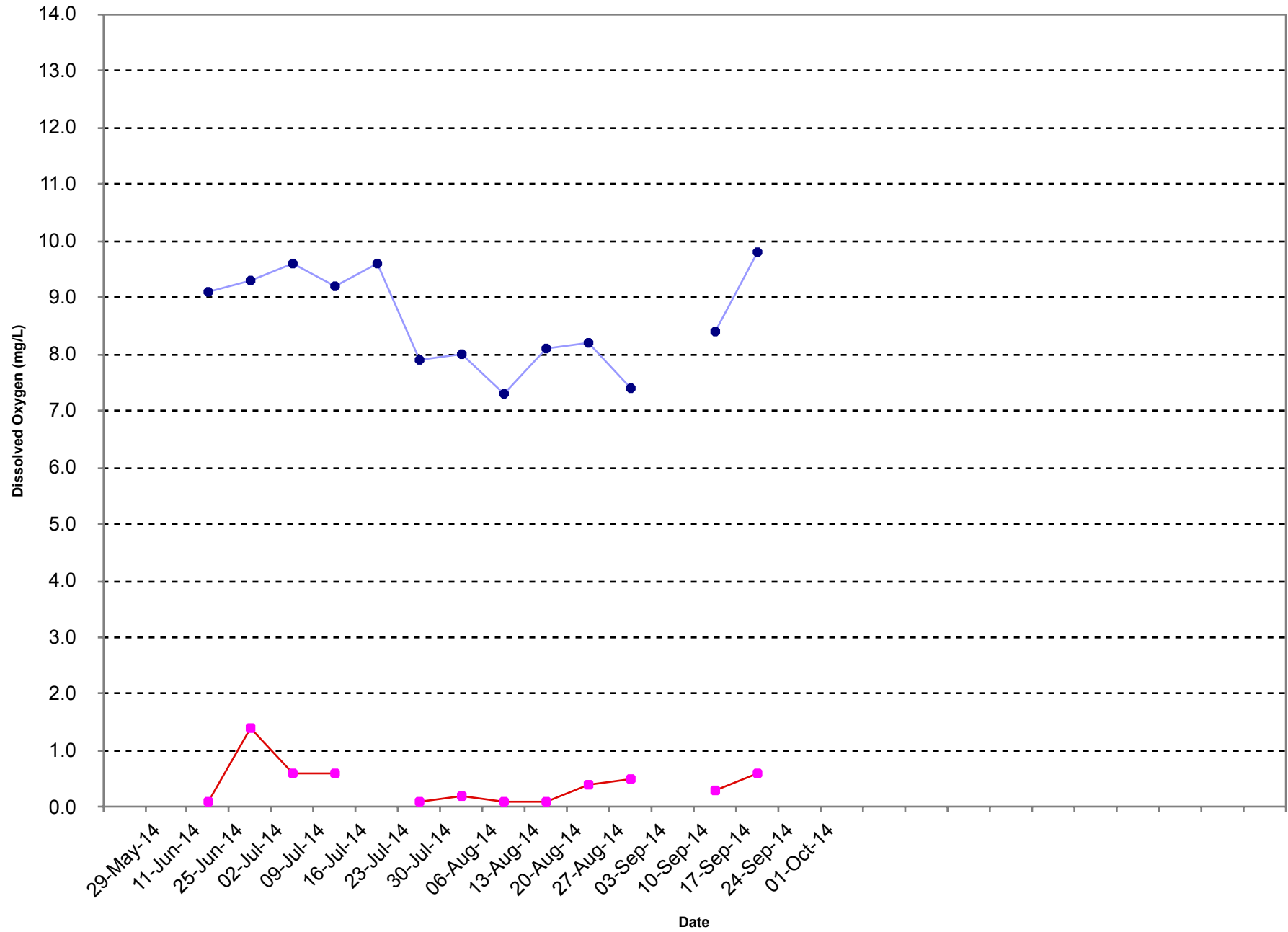
Osoyoos Lake (at Central Basin) - Dissolved Oxygen
