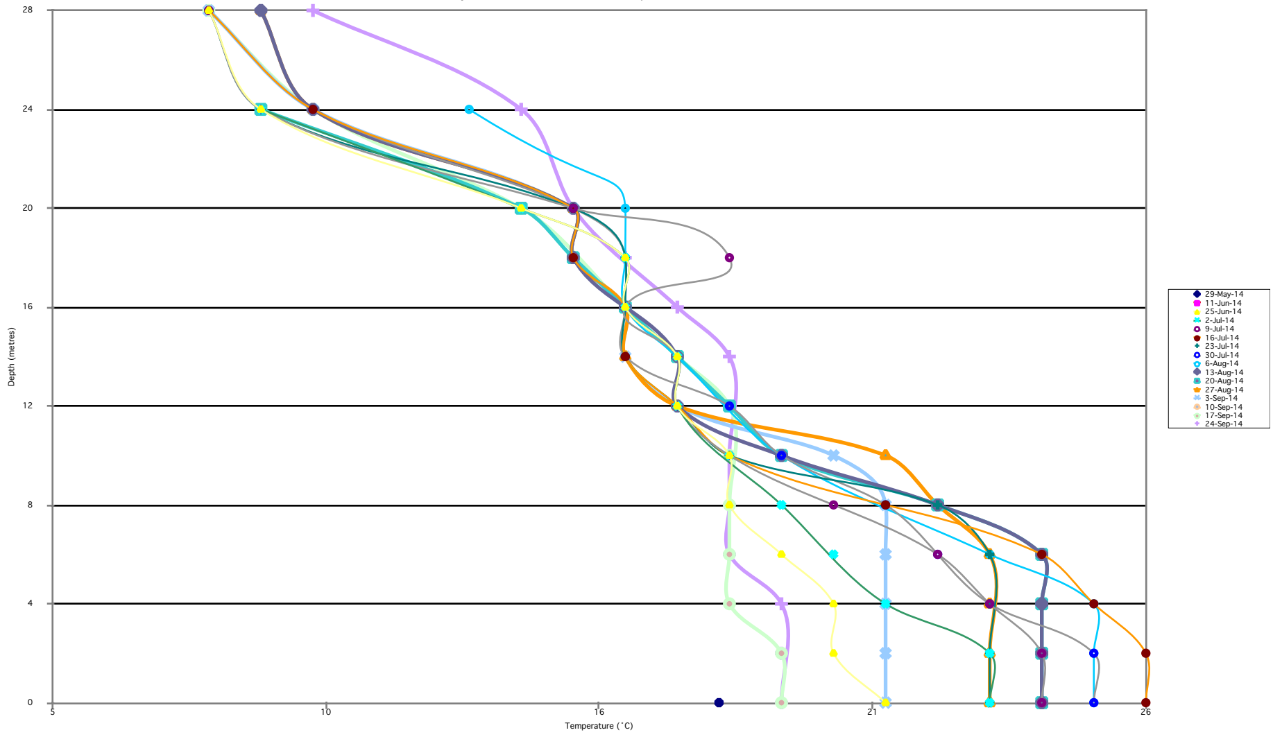
Osoyoos Lake (at Central Basin) - Temperature Profiles 2014
