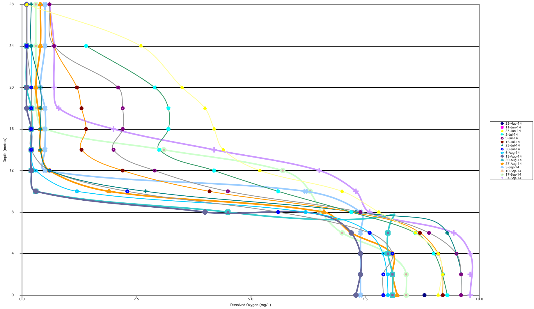
Osoyoos Lake (at Central Basin) - Oxygen Profiles 2014
