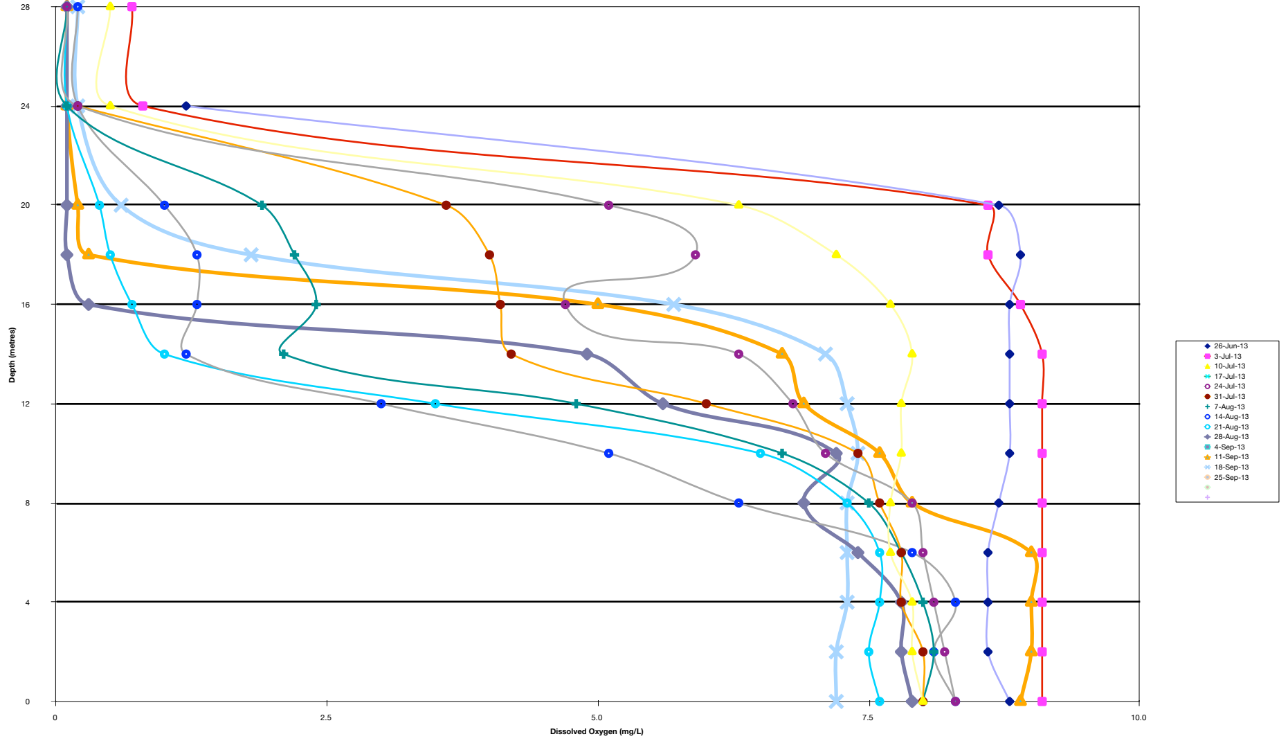
Osoyoos Lake (at Central Basin) - Oxygen Profiles 2013
